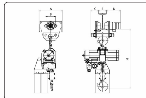
Hoist with trolley
